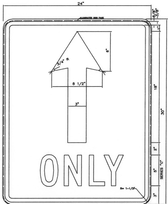
ILLUMINATED SIGN FACE ILLUM. SIGN FACE 1/4" SMALLER THAN REFL. OMIT BORDER BLACK SYMBOL & LEGEND WHITE BACKGROUND
