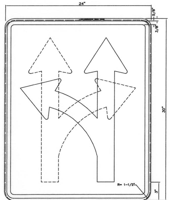
ILLUMINATED SIGN FACE ILLUM. SIGN FACE 1/4" SMALLER THAN REFL. OMIT BORDER BLACK SYMBOL & LEGEND WHITE BACKGROUND
