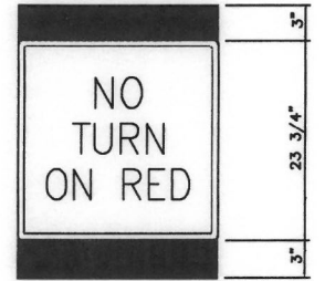
SPECIAL 24"x 30" (NOMINAL) ILLUMINATED SIGN FACE
