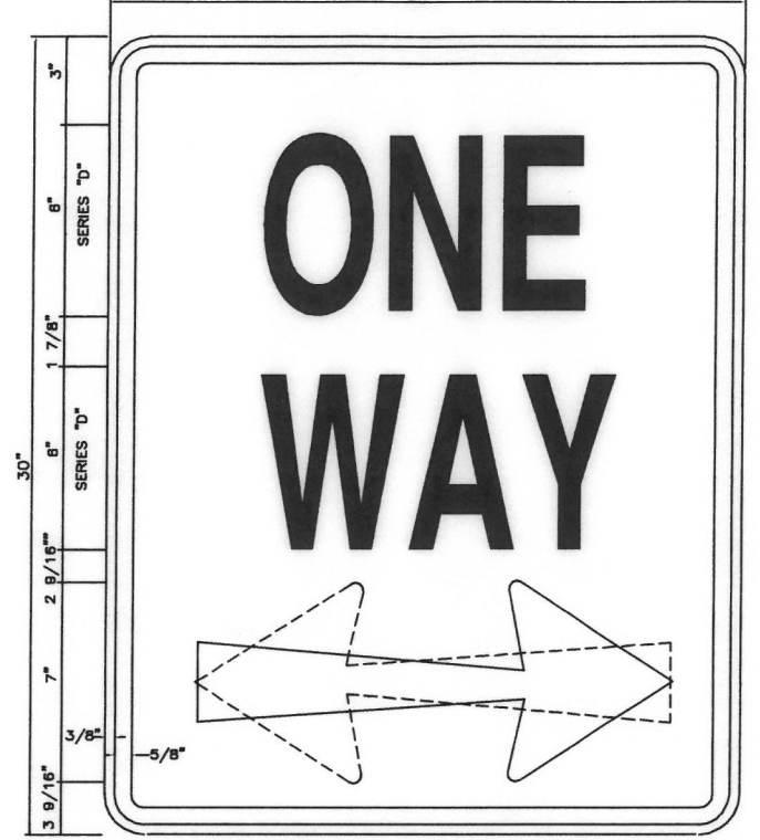
BLACK SYMBOL & LEGEND WHITE BACKGROUND CITY # 92 A,C
