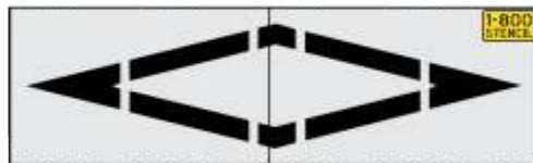
MUTCD Preferential Lane Symbol 156" x 40"
