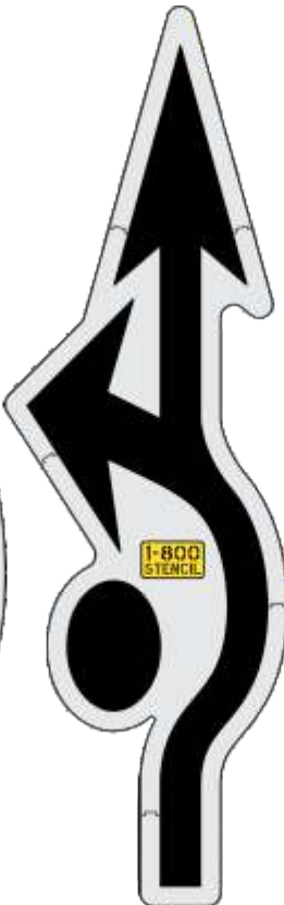
Roundabout Fish Hook Arrow Straight Left 252" x 72"
