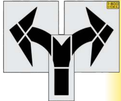
MUTCD Left/Right Combo Arrow 91" x 77"
