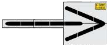
MUTCD Wrong Way Arrow 280" x 98"
