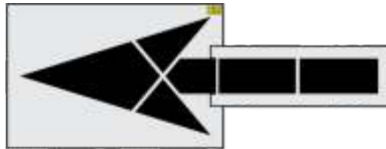
MUTCD Straight Arrow 42" x 120"
