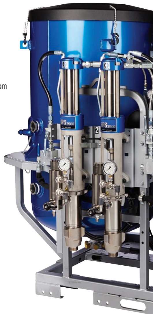
2-Pump RoadPak
